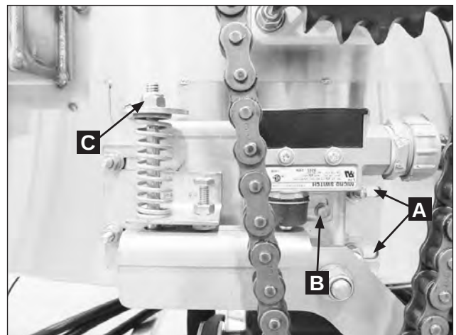
Anti-jam Switch
